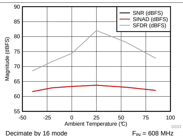
Figure 6. SNR, SINAD, SFDR vs Temperature
