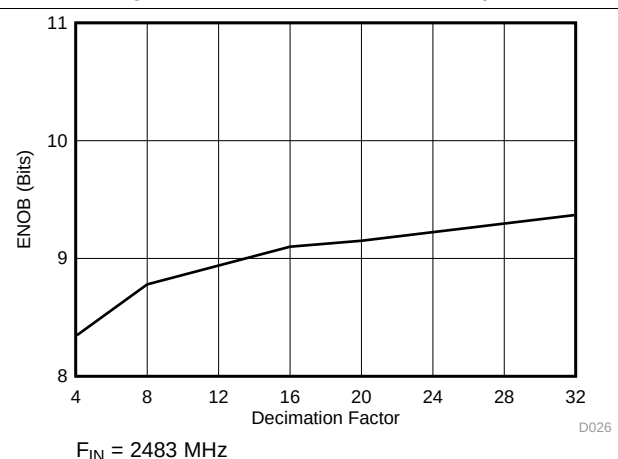
Figure 8. ENOB vs Decimation Setting
