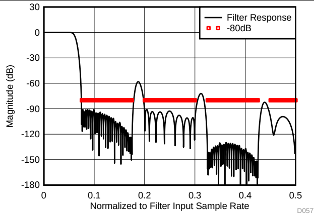
Figure 21. Decimate by 8 - Stopband Response
