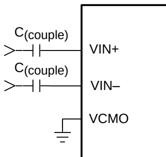
Figure 32. Differential Analog Input Connection
