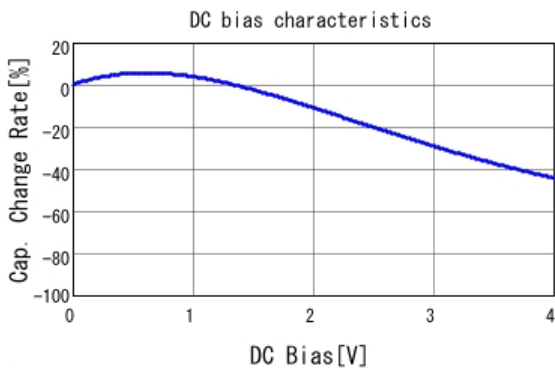
■ LLR185C70G105ME05 C-DC bias capchange, 25.0degC, AC0.
