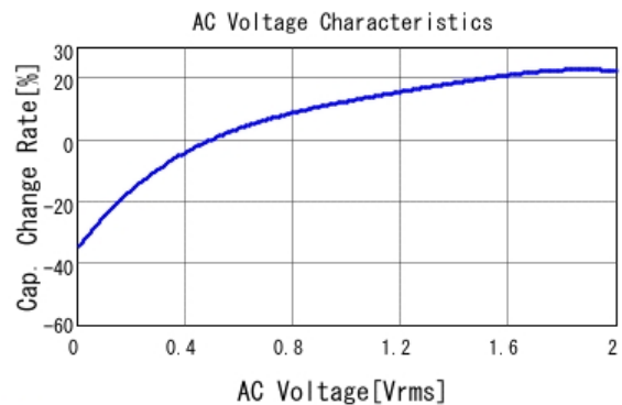
■ LLR185C70G105ME05 C-AC Voltage capchange, DC0V, 25.0d
