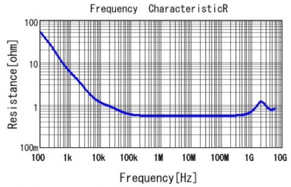
■ LLR185C70G105ME05 R DC0V, 25degC
