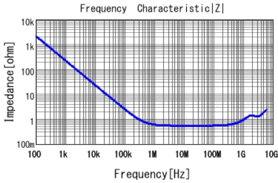
■ LLR185C70G105ME05 |Z| DC0V, 25degC
