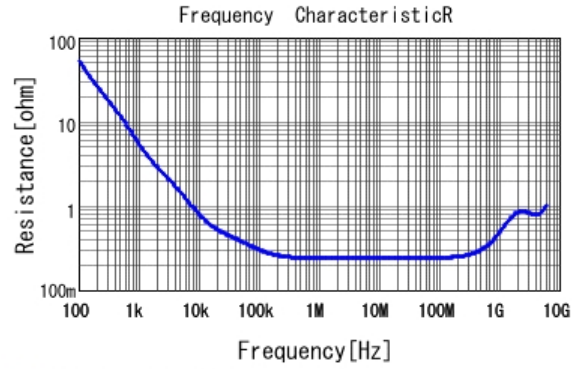
■ LLR185C70G105ME03 R DC0V, 25degC
