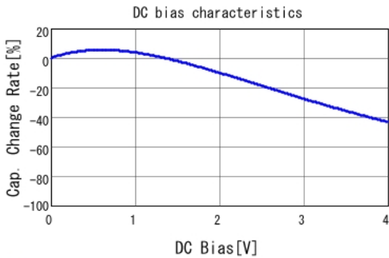
■ LLR185C70G105ME03 C-DC bias capchange, 25.0degC, AC0.
