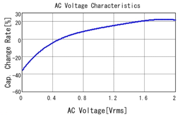
■ LLR185C70G105ME03 C-AC Voltage capchange, DC0V, 25.0d
