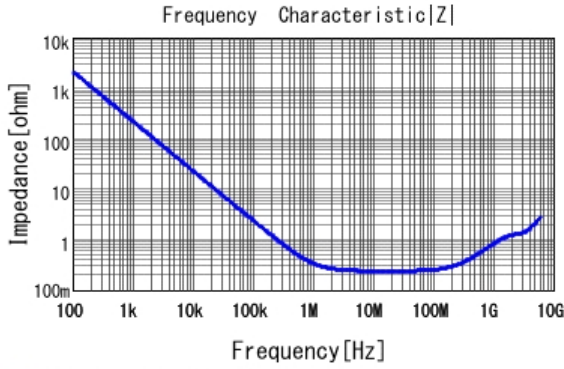
■ LLR185C70G105ME03 |Z| DC0V, 25degC
