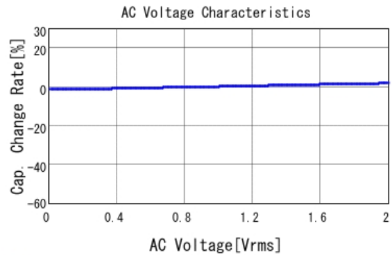
■ LLL185R71H472MA01 C-AC Voltage capchange, DC0V, 25.0d
