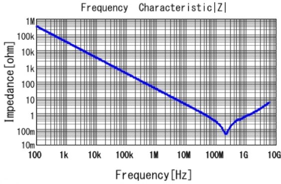
■ LLL185R71H472MA01 |Z| DC0V, 25degC
