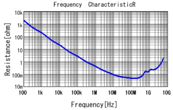
■ LLL185R71H472MA01 R DC0V, 25degC
