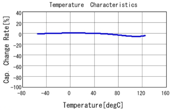
■ LLL185R71H472MA01 C-Temp. capchange, DC0.0V, AC1.0Vrm
