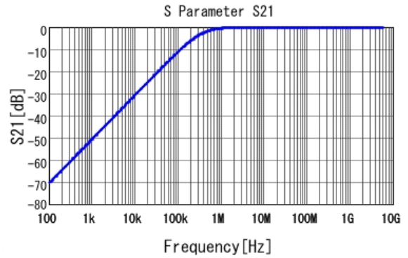
■ LLL185R71H472MA01 S21 DC0V, 25degC
