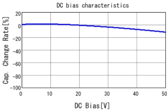
■ LLL185R71H472MA01 C-DC bias capchange, 25.0degC, AC1.
