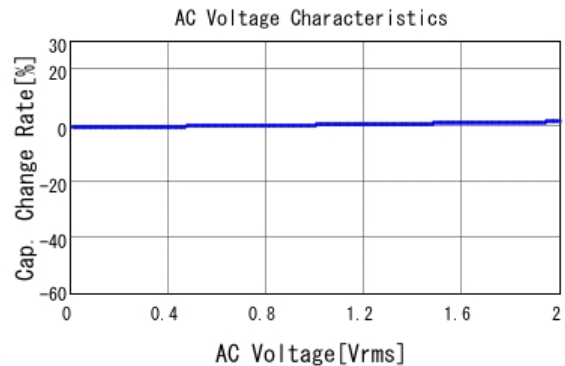
■ LLL185R71H222MA01 C-AC Voltage capchange, DCOV, 25.0d
