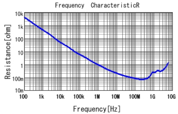
■ LLL185R71H222MA01 R DCOV, 25degC
