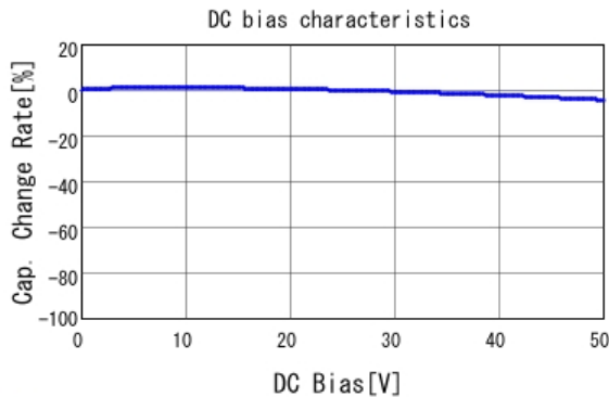
■ LLL185R71H222MA01 C-DC bias capchange, 25.0degC, AC1.
