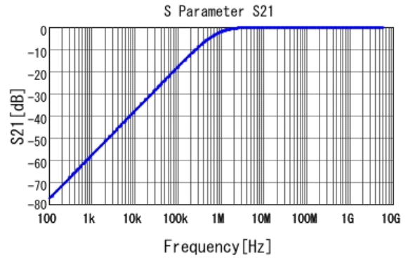
■ LLL185R71H222MA01 S21 DC0V, 25degC
