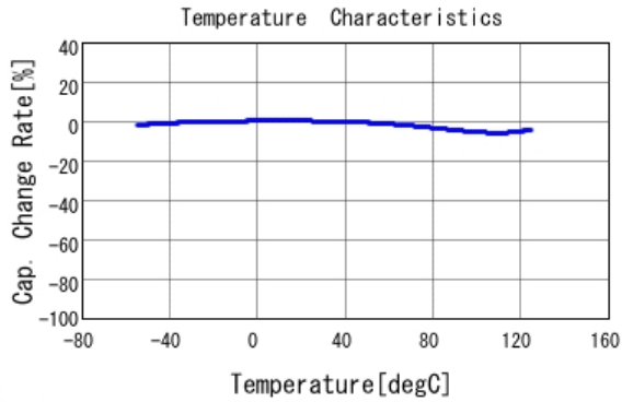
■ LLL185R71H222MA01 C-Temp. capchange, DC0.0V, AC1.0Vrm
