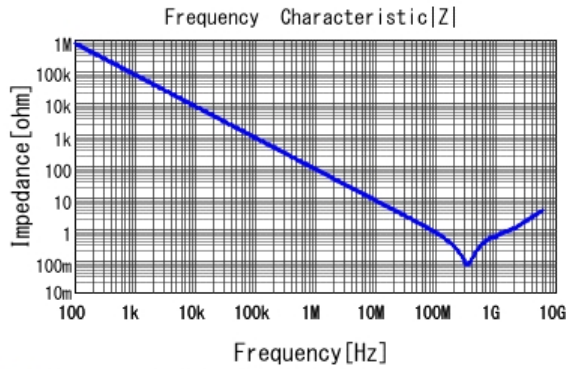
■ LLL185R71H222MA01 |Z| DCOV, 25degC
