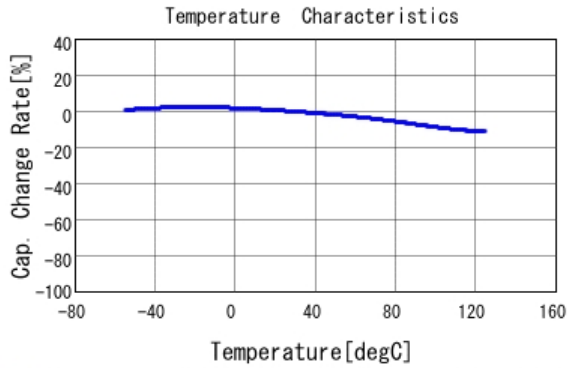
■ LLL185R71C473MA01 C-Temp. capchange, DC0.0V, AC1.0Vrm
