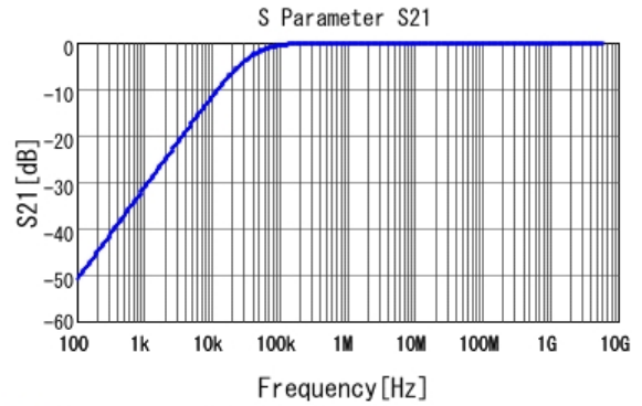
■ LLL185R71C473MA01 S21 DC0V, 25degC
