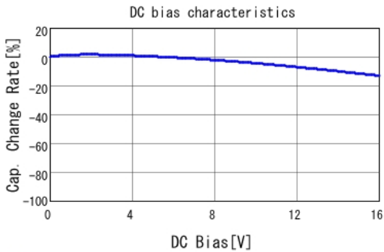
■ LLL185R71C223MA11 C-DC bias capchange, 25.0degC, AC1.
