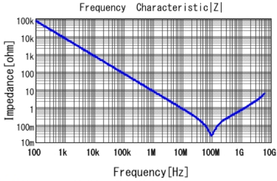
■ LLL185R71C223MA11 |Z| DCOV, 25degC
