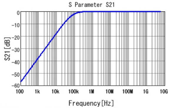
■ LLL185R71C223MA11 S21 DC0V, 25degC
