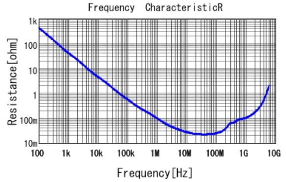
■ LLL185R71C223MA11 R DCOV, 25degC
