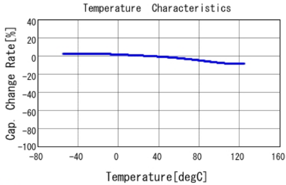
■ LLL185R71C223MA11 C-Temp. capchange, DC0.0V, AC1.0Vrm
