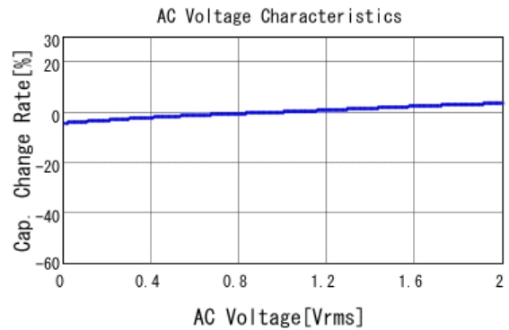
■ LLL185R71C223MA11 C-AC Voltage capchange, DCOV, 25.0d
