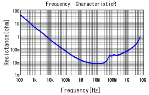
■ LLL185R71A224MA01 R DCOV, 25degC
