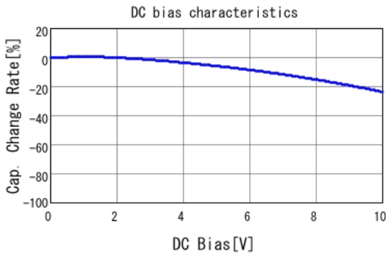
■ LLL185R71A224MA01 C-DC bias capchange, 25.0degC, AC1.
