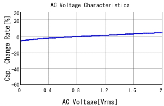
■ LLL185R71A224MA01 C-AC Voltage capchange, DCOV, 25.0d
