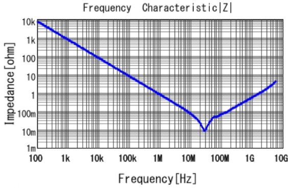
■ LLL185R71A224MA01 |Z| DCOV, 25degC
