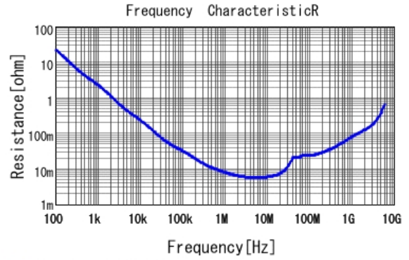
■ LLL185C70G474MA01 R DC0V, 25degC
