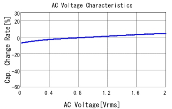
■ LLL185C70G474MA01 C-AC Voltage capchange, DC0V, 25.0d
