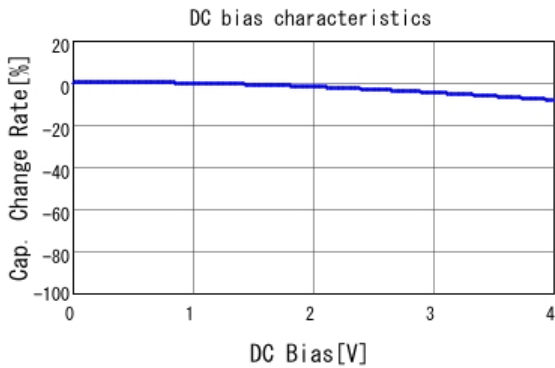
■ LLL185C70G474MA01 C-DC bias capchange, 25.0degC, AC1.
