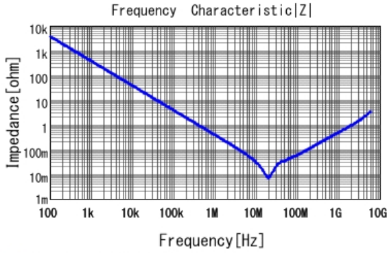
■ LLL185C70G474MA01 |Z| DC0V, 25degC
