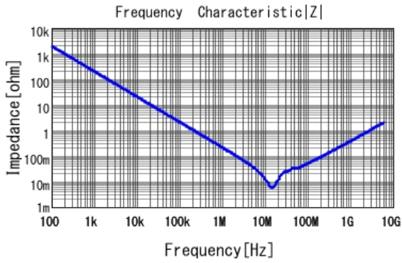
■ LLL153C70E105ME21 |Z| DC0V, 25degC
