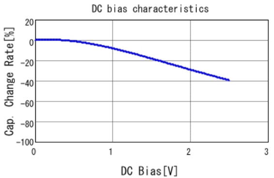
■ LLL153C70E105ME21 C-DC bias capchange, 25.0degC, AC0.
