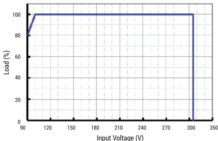
Derating Curve
