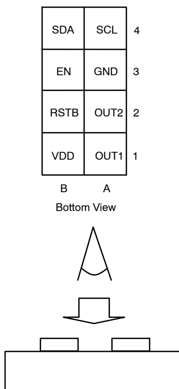
Figure 2. Pin Layout
