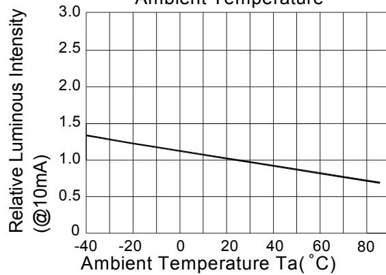
Intensity VS. Ambient Temperature
