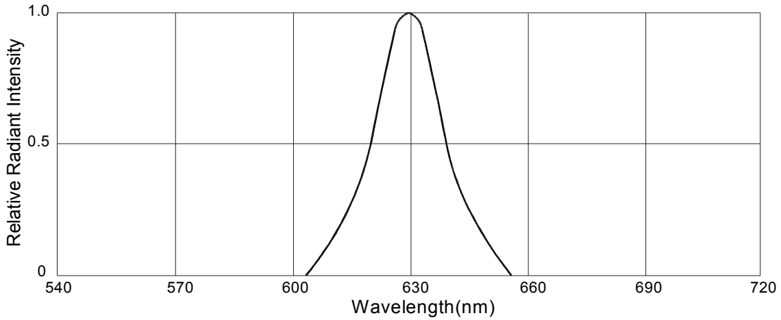
Fig.1 Relative Radiant Intensity VS. Wavelength
