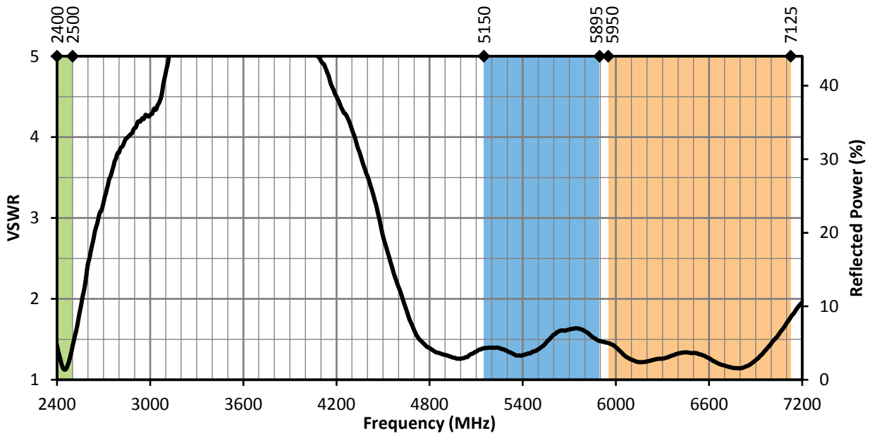
Figure 2. ANT-W63-FPC-SH Antenna VSWR with Frequency Band Highlights
