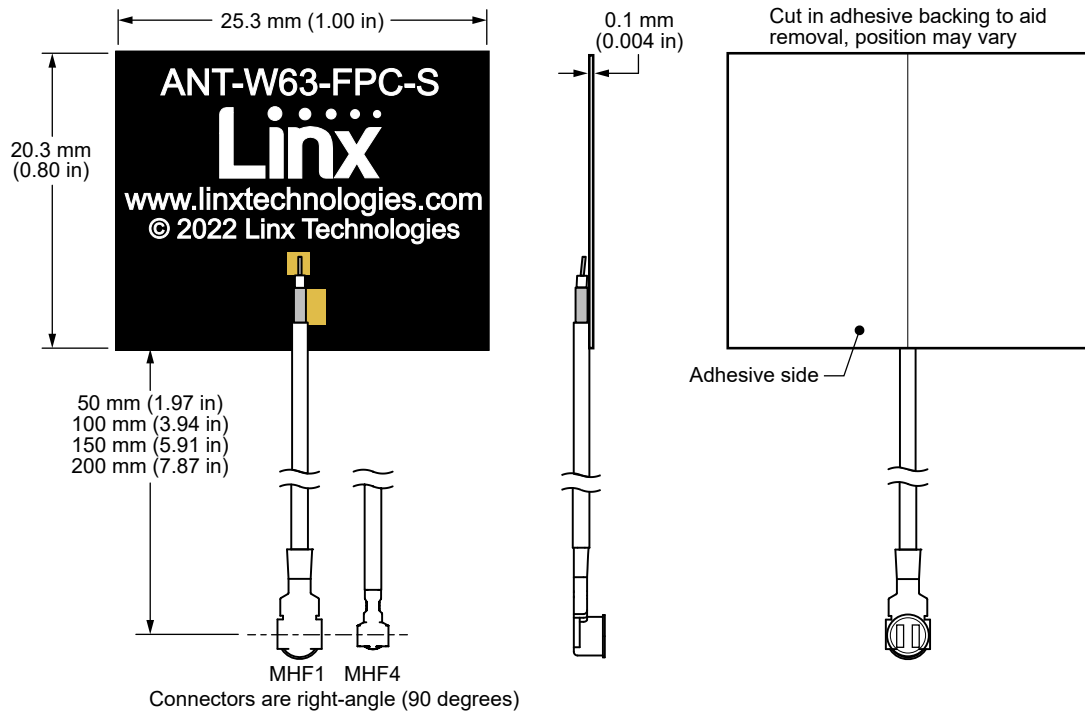
Figure 1. ANT-W63-FPC-SH Series Antenna Dimensions
