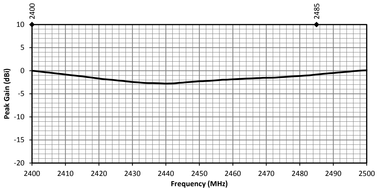
Figure 4. ANT-2.4-FPC-SAH Antenna Peak Gain
