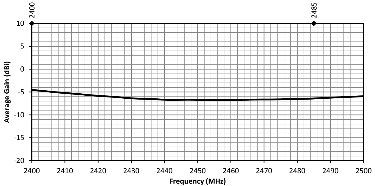
Figure 5. ANT-2.4-FPC-SAH Antenna Average Gain
