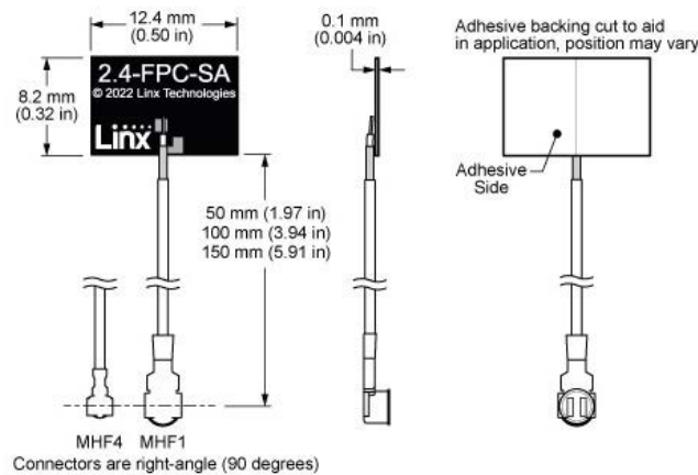
Figure 1. ANT-2.4-FPC-LV Series Antenna Dimensions
