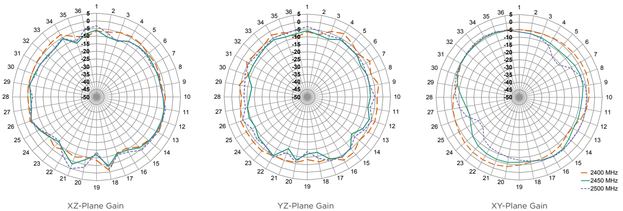
Figure 7. Radiation Patterns for ANT-2.4-FPC-SAH Series Antenna
