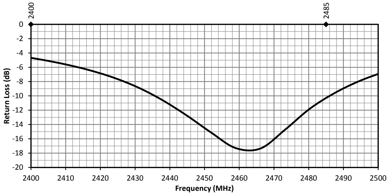
Figure 3. ANT-2.4-FPC-SAH Antenna Return Loss
