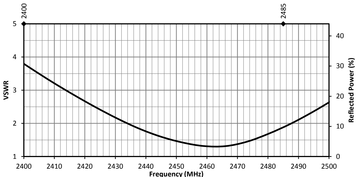
Figure 2. ANT-2.4-FPC-SAH Antenna VSWR
