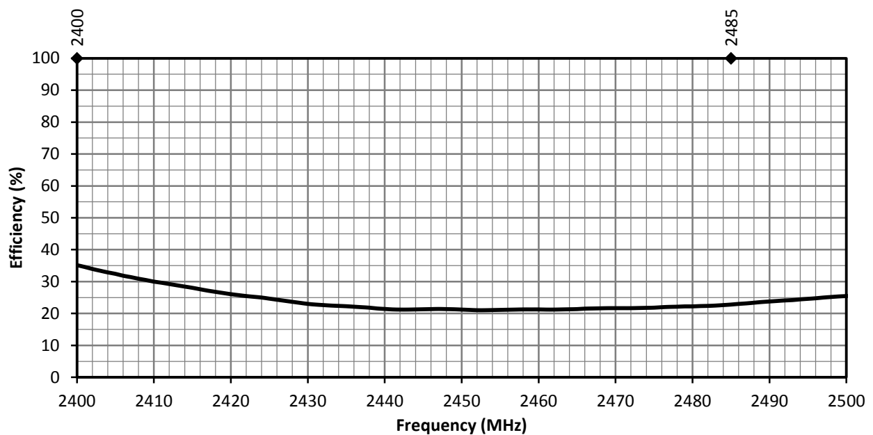
Figure 6. ANT-2.4-FPC-SAH Antenna Radiation Efficiency
