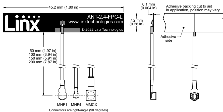
Figure 1. ANT-2.4-FPC-LH Series Antenna Dimensions
