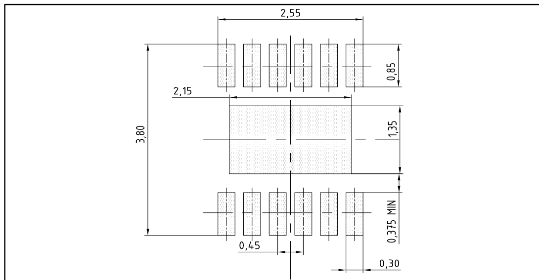
Figure 18: VFDFPN 12L (3x3x0.90 mm) recommended footprint
