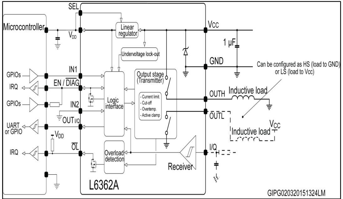
Figure 16: Inductive load driver
