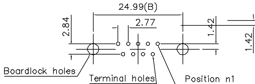
Recomended PCB Layout
