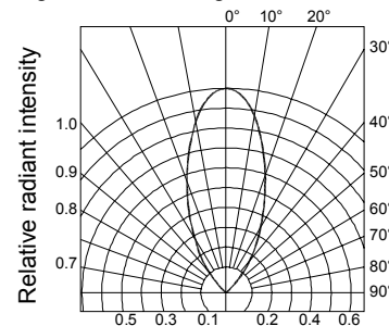
Fig.6 Radiation diagram
