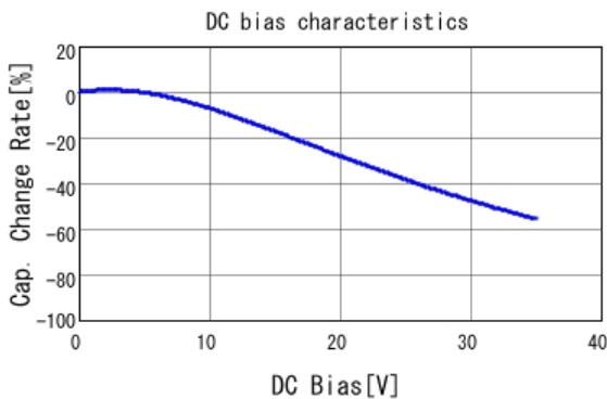
■ KRM55WR7YA476MH01 C-DC bias capchange, 25.0degC, AC0.
