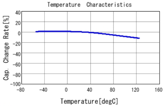
■ KRM55WR7YA476MH01 C-Temp. capchange, DCOV, ACO, 5Vrms
