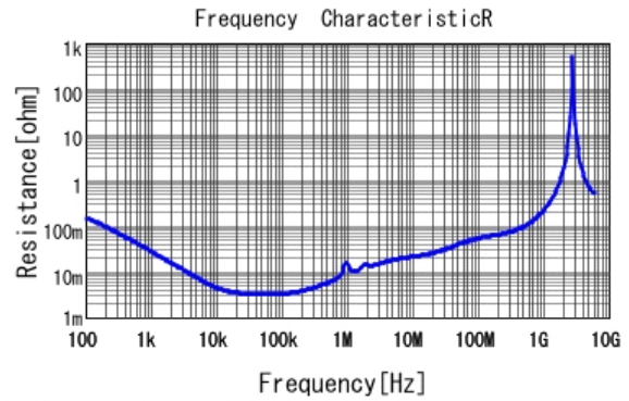
■ KRM55WR7YA476MH01 R DCOV, 25degC
