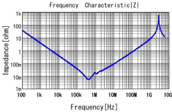
■ KRM55WR7YA476MH01 |Z| DCOV, 25degC
