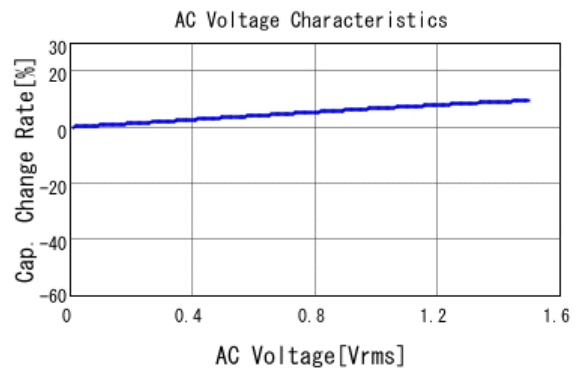
■ KRM55WR7YA476MH01 C-AC Voltage capchange, DCOV, 25.0d
