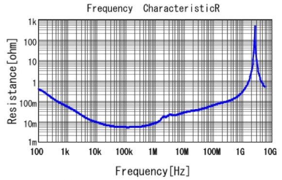
■ KRM55QR7YA226KH01 R DC0V, 25degC
