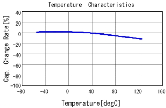
■ KRM55QR7YA226KH01 C-Temp. capchange, DCOV, ACO, 5Vrms
