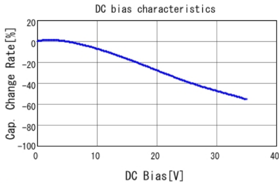
■ KRM55QR7YA226KH01 C-DC bias capchange, 25.0degC, AC0.
