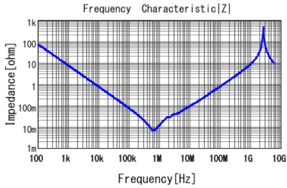
■ KRM55QR7YA226KH01 |Z| DC0V, 25degC
