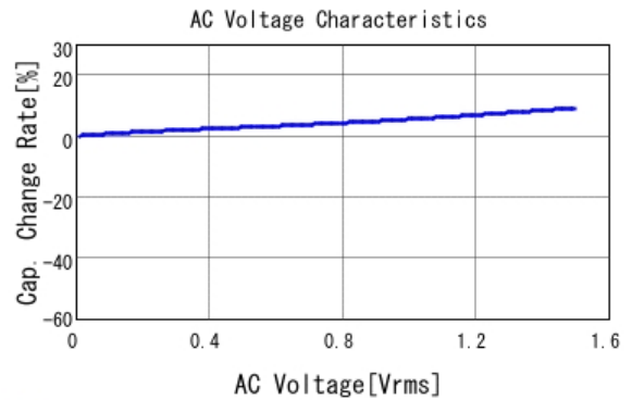
■ KRM55QR7YA226KH01 C-AC Voltage capchange, DC0V, 25.0d
