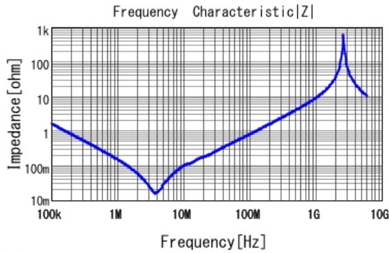
■ KRM55LR72E105KH01 |Z| DC0V, 25degC
