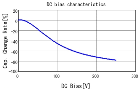
■ KRM55LR72E105KH01 C-DC bias capchange, 25.0degC, AC1V
