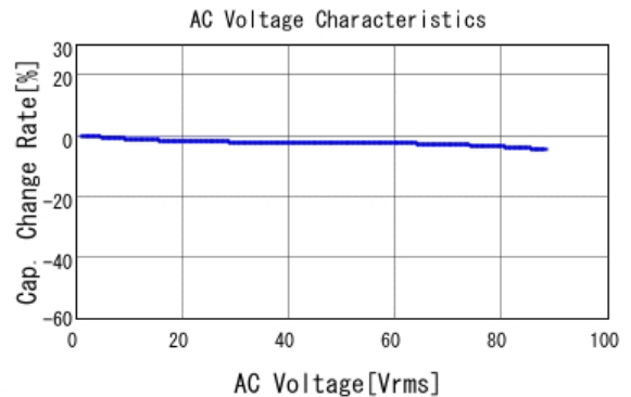
■ KRM55LR72E105KH01 C-AC Voltage capchange, DC0V, 25.0d
