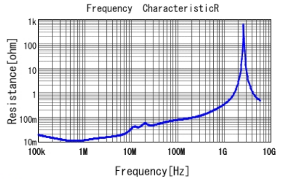
■ KRM55LR72E105KH01 R DC0V, 25degC
