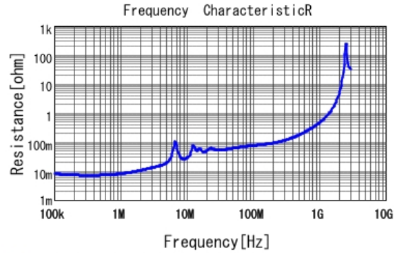
■ KR355WD72W125MH01 R DC0V, 25degC
