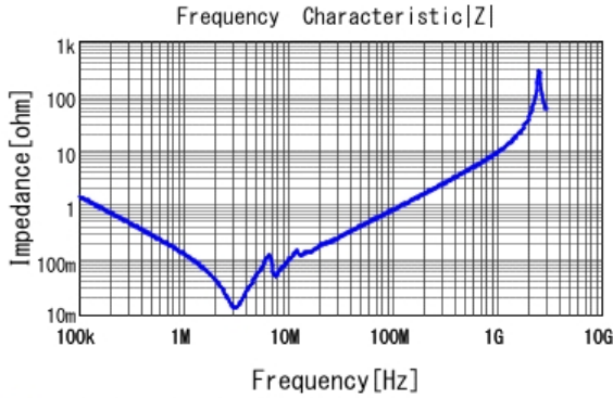
■ KR355WD72W125MH01 |Z| DC0V, 25degC
