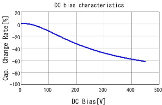
■ KR355WD72W125MH01 C-DC bias capchange, 25.0degC, AC1V
