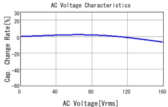
■ KR355WD72W125MH01 C-AC Voltage capchange, DC0V, 25.0d
