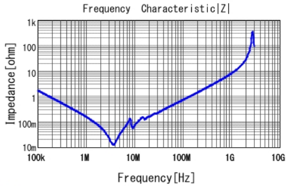
■ KR355TD72W105MH01 |Z| DC0V, 25degC
