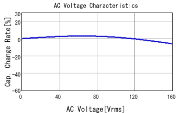
■ KR355TD72W105MH01 C-AC Voltage capchange, DC0V, 25.0d
