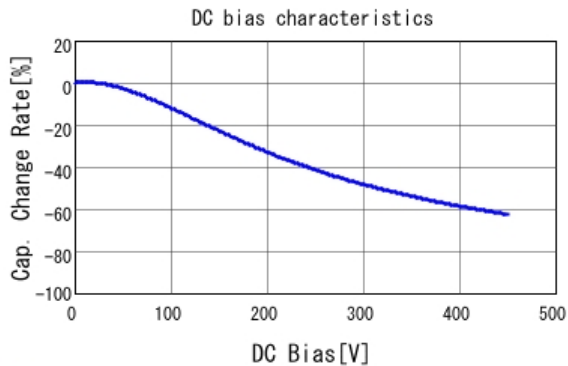
■ KR355TD72W105MH01 C-DC bias capchange, 25.0degC, AC1V
