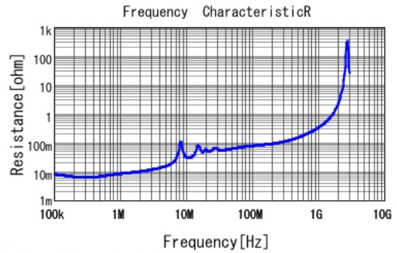
■ KR355TD72W105MH01 R DC0V, 25degC
