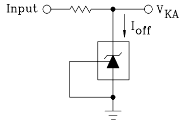
FIGURE 3—TEST CIRCUIT FOR I_{off}
