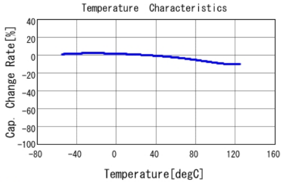
■ KCM55WR71E686MH01 C-Temp. capchange, DCOV, ACO, 5Vrms
