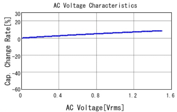
■ KCM55WR71E686MH01 C-AC Voltage capchange, DCOV, 25.0d
