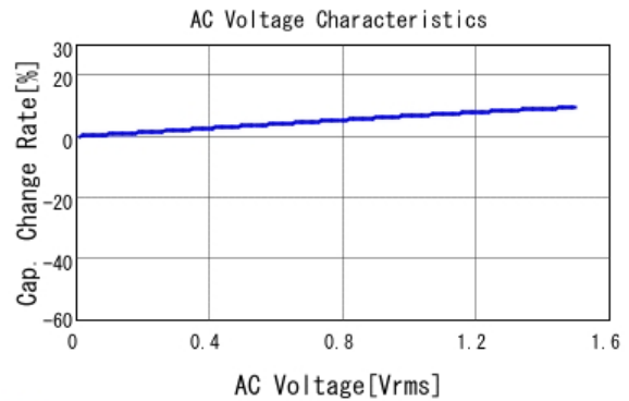
■ KCM55WR71E476MH01 C-AC Voltage capchange, DCOV, 25.0d
