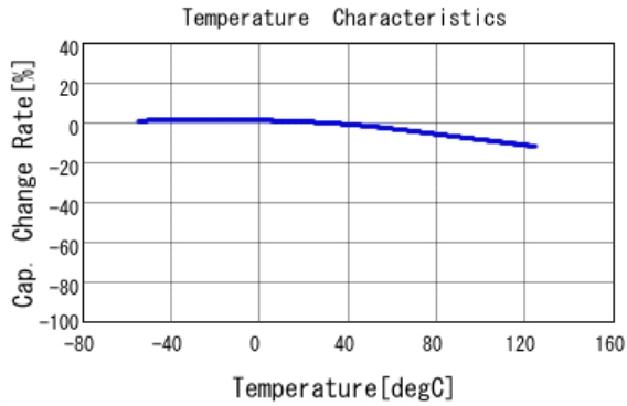
■ KCM55WR71E476MH01 C-Temp. capchange, DCOV, ACO, 5Vrms
