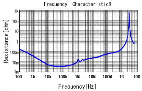
■ KCM55WR71E476MH01 R DCOV, 25degC
