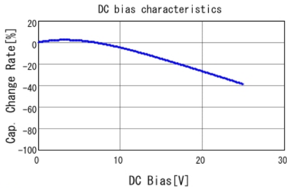
■ KCM55WR71E476MH01 C-DC bias capchange, 25.0degC, AC0.
