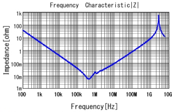
■ KCM55WR71E476MH01 |Z| DCOV, 25degC
