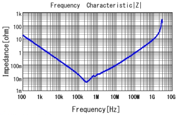
■ KCM55WC71E107MH13 |Z| DC0V, 25degC
