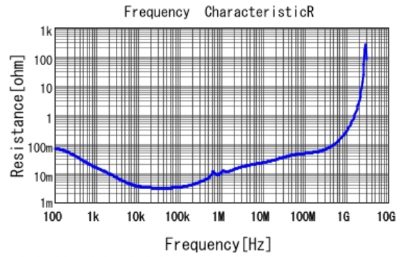
■ KCM55WC71E107MH13 R DC0V, 25degC
