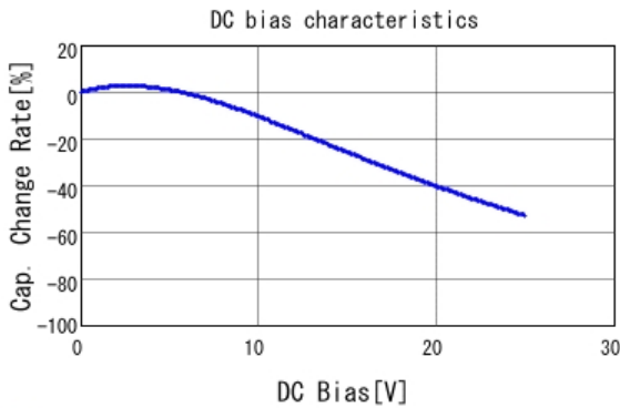
■ KCM55WC71E107MH13 C-DC bias capchange, 25.0degC, AC0.
