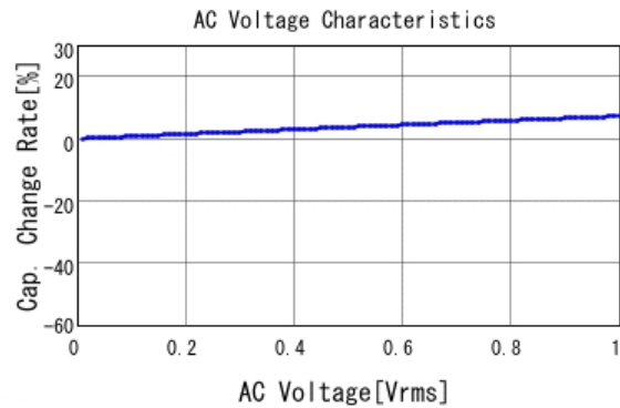
■ KCM55WC71E107MH13 C-AC Voltage capchange, DC0V, 25.0d
