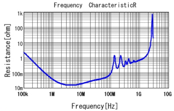
■ KCA55Q7UMF472KL01 R DC0V, 25degC
