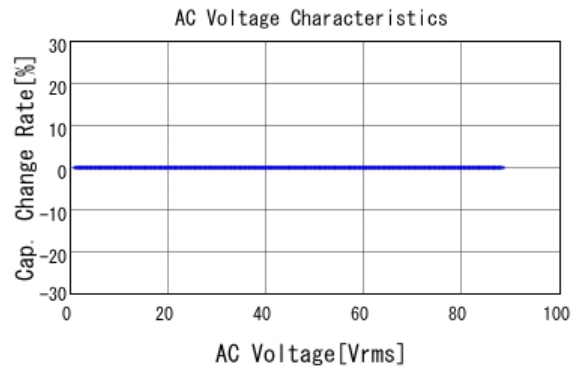
■ KCA55Q7UMF472KH01 C-AC Voltage capchange, DC0V, 25.0d
