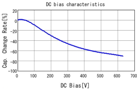
■ KC355WD7LQ125MV01 C-DC bias capchange, 25.0degC, AC1V
