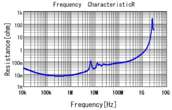
■ KC355WD7LQ125MV01 R DC0V, 25degC
