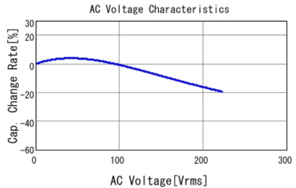
■ KC355WD7LQ125MV01 C-AC Voltage capchange, DC0V, 25.0d
