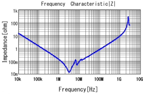
■ KC355WD7LQ125MV01 |Z| DC0V, 25degC
