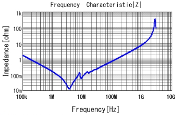
■ KC355TD7LQ105MV01 |Z| DC0V, 25degC
