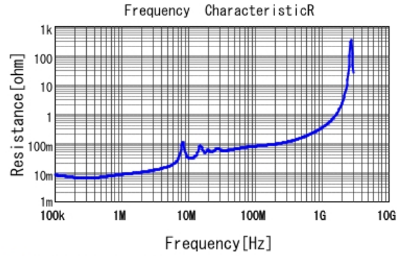
■ KC355TD7LQ105MV01 R DC0V, 25degC
