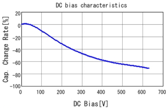
■ KC355TD7LQ105MV01 C-DC bias capchange, 25.0degC, AC1V
