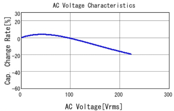
■ KC355TD7LQ105MV01 C-AC Voltage capchange, DC0V, 25.0d
