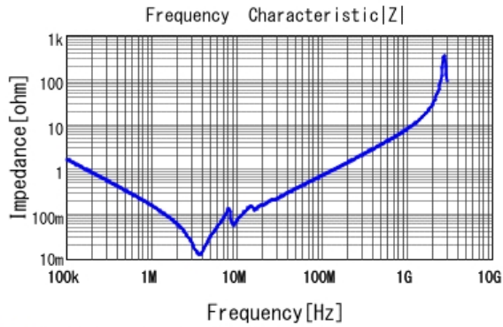
■ KC355TD72W105MH01 |Z| DC0V, 25degC
