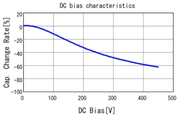
■ KC355TD72W105MH01 C-DC bias capchange, 25.0degC, AC1V
