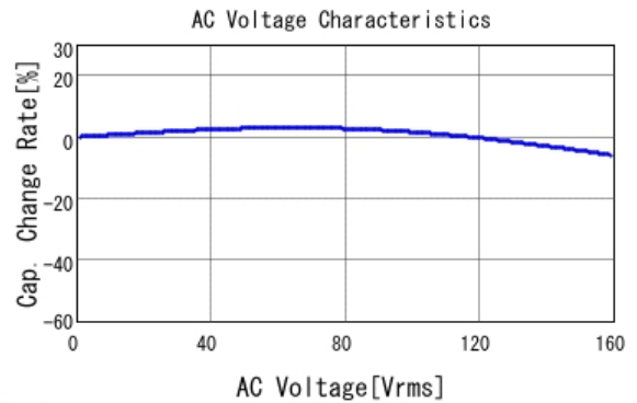
■ KC355TD72W105MH01 C-AC Voltage capchange, DC0V, 25.0d
