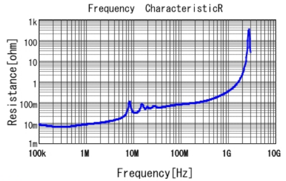
■ KC355TD72W105MH01 R DC0V, 25degC
