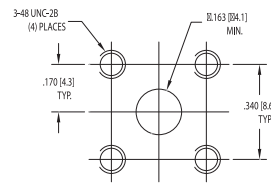
MOUNTING HOLE C
