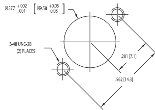
MOUNTING HOLE F
