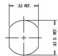
MOUNTING HOLE AO
