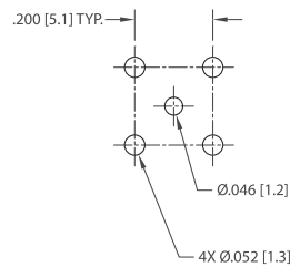
MOUNTING HOLE O
