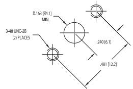
MOUNTING HOLE D
