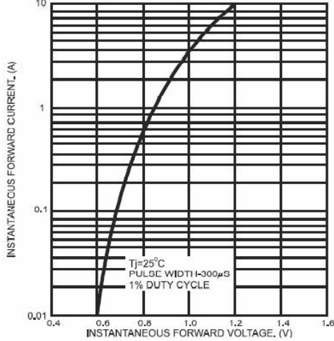
FIG.5- TYPICAL FORWARD CHARACTERISTICS PER BRIDGE ELEMENT
