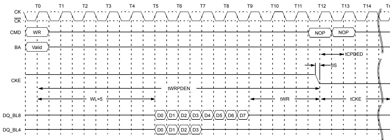
Figure 91. Power-Down Entry after Write
