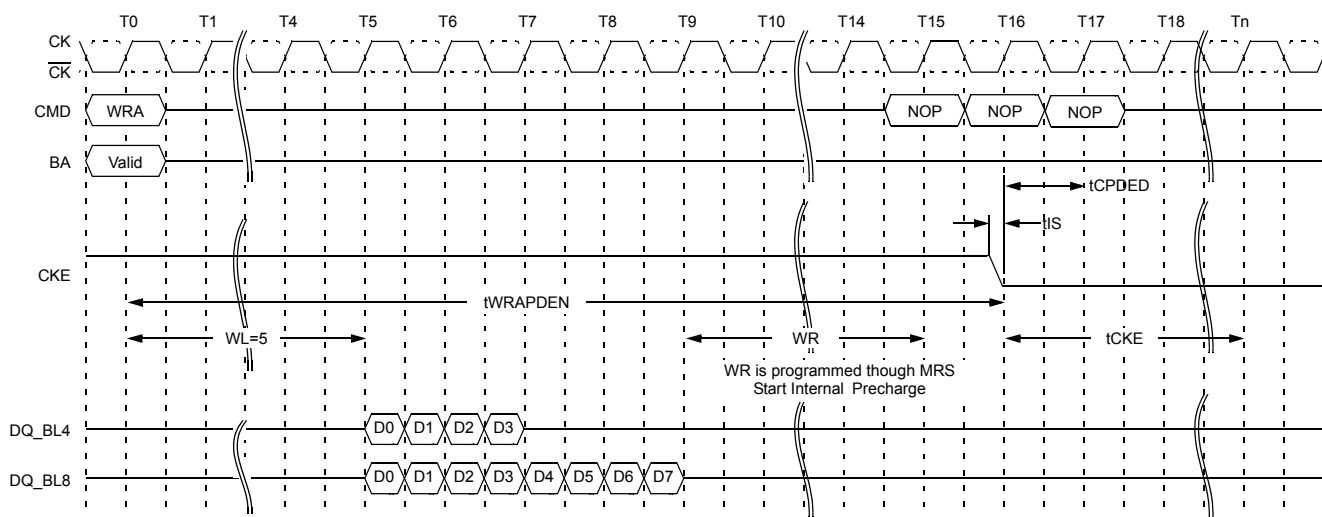
Figure 90. Power-Down Entry After Write with Auto Precharge
