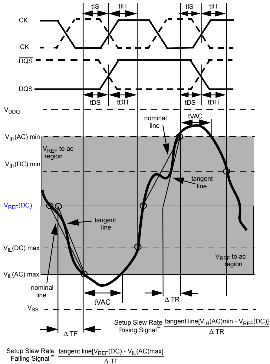
Figure 23. Illustration of tangent line for setup time t DS (for DQ with respect to strobe) and t S (for ADD/CMD with respect to clock)
