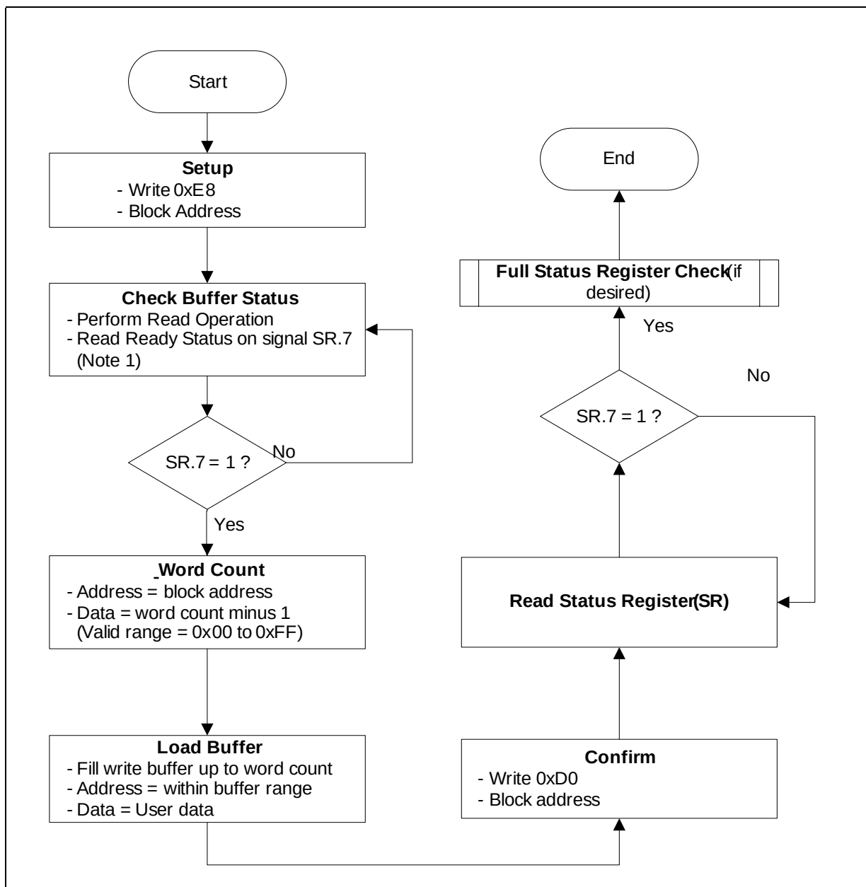
Figure 16: Write to Buffer Flowchart
