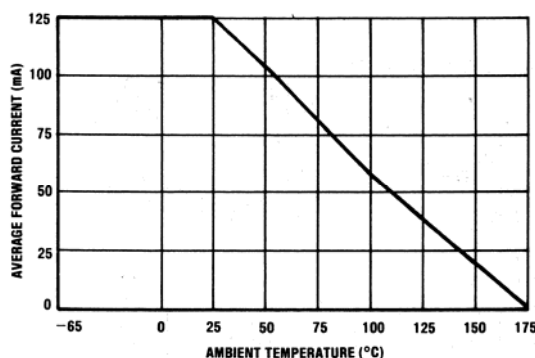
FIGURE 2 1N5181-84
