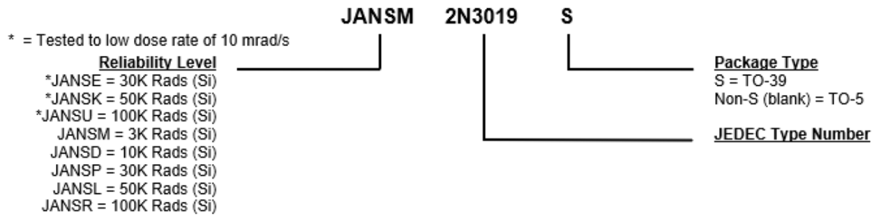
Figure 2-1. Part Nomenclature
