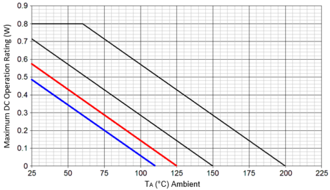
Figure 4-2. Temperature-Power Derating ( R_{\Theta JS} )
