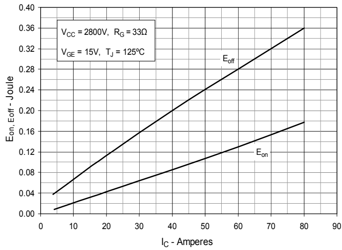
Fig. 12. Typ. Swicthng Characteristics vs. Collector Current
