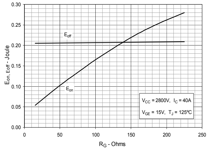
Fig. 13. Typ. Swicthng Characteristics vs. Gate Resistor
