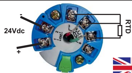
RTD 3-WIRE
