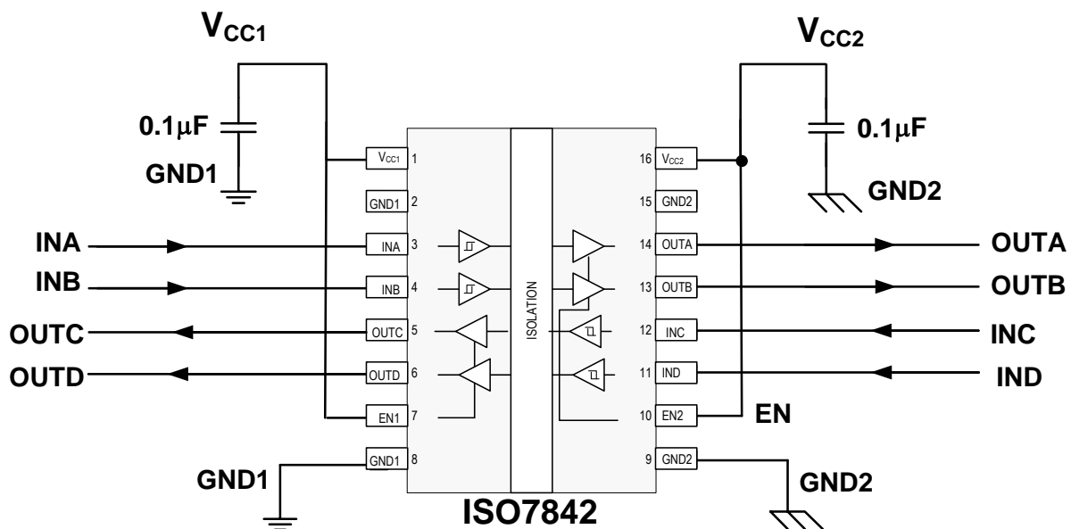
Figure 16. Typical ISO7842 Circuit Hook-up
