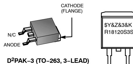
D²PAK-3 (TO-263, 3-LEAD) CASE 418AJ
