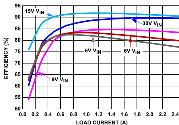
FIGURE 26. EFFICIENCY, BOOST BUCK, 500kHz, V_{OUT} = 12V , T_A = +25^\circ C
