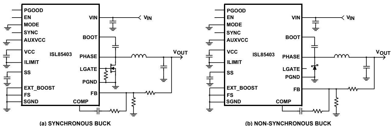
FIGURE 3. TYPICAL APPLICATION SCHEMATIC I
