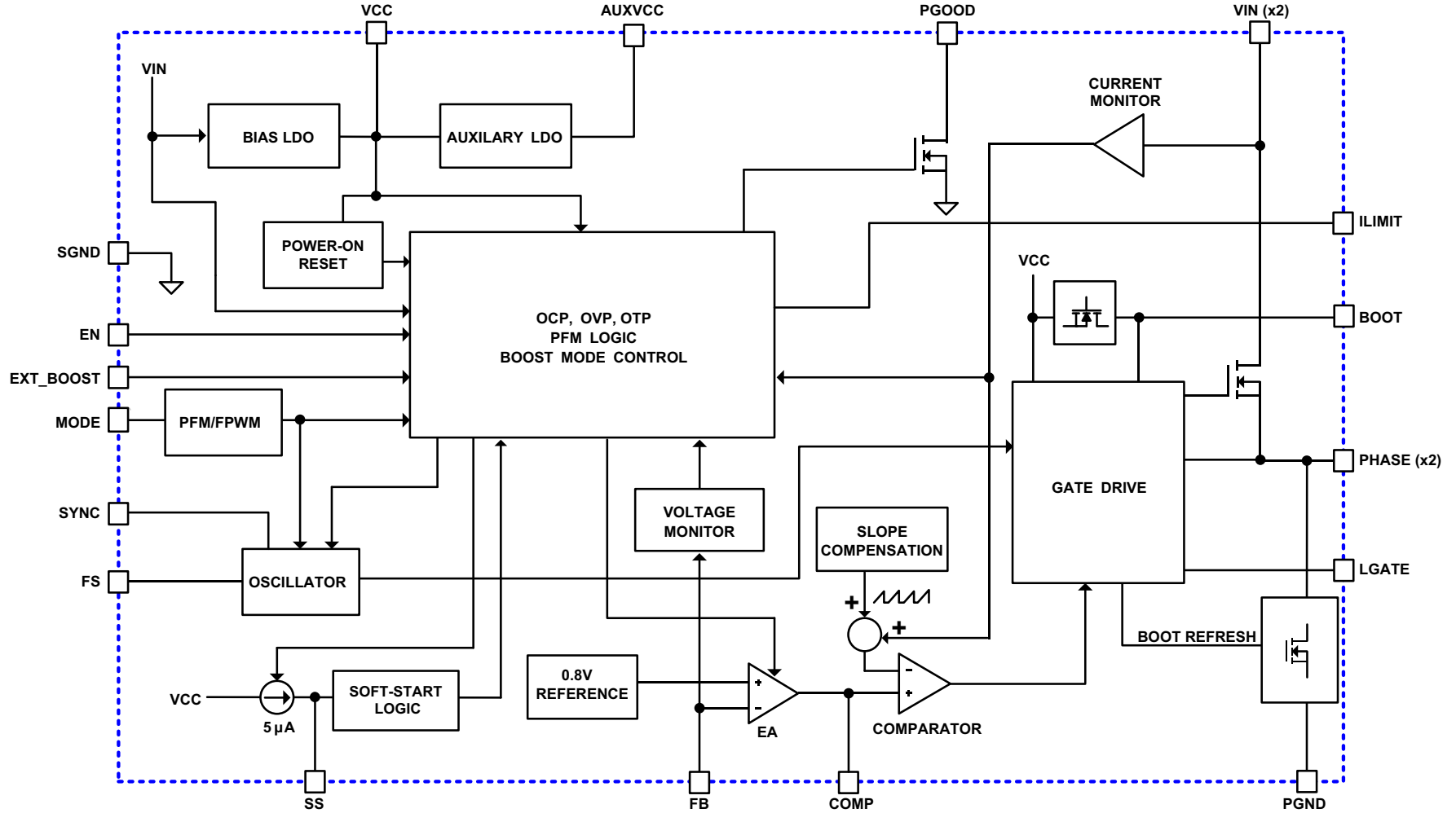
FIGURE 6. BLOCK DIAGRAM
