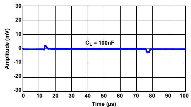
Figure 13. Line Transient with 100nF Load ( \Delta V_{IN} = \pm 500\text{mV} )
