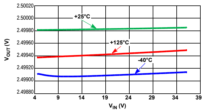
Figure 10. Line Regulation, Three Temperatures
