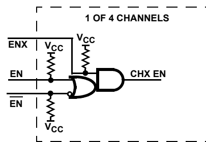
FIGURE 33. ISL32x77E ENABLE LOGIC
