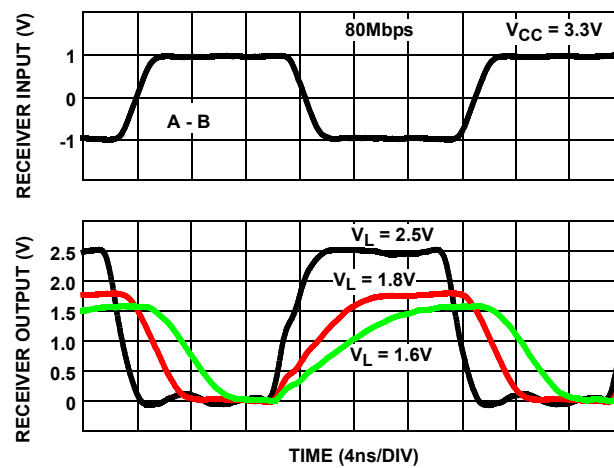
FIGURE 31. ISL32177E RECEIVER WAVEFORMS
