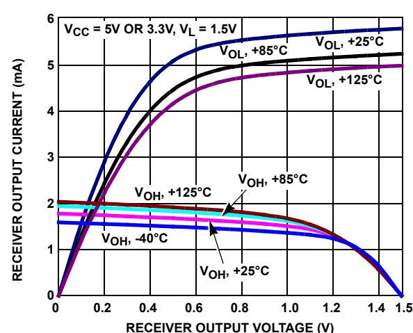
FIGURE 19. ISL32277E RECEIVER OUTPUT CURRENT vs RECEIVER OUTPUT VOLTAGE
