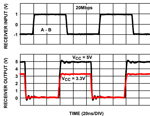
FIGURE 29. ISL3227xE RECEIVER WAVEFORMS
