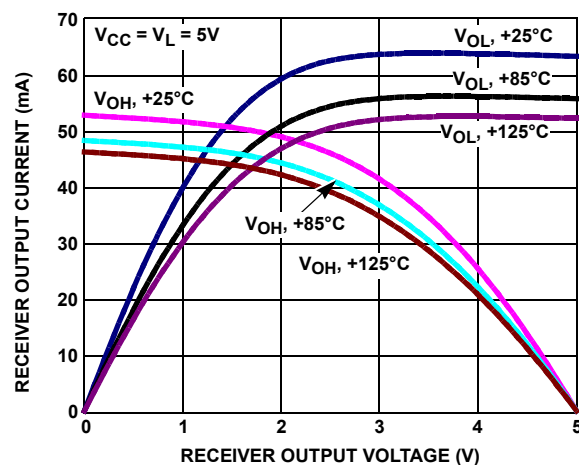
FIGURE 15. ISL3227xE RECEIVER OUTPUT CURRENT vs RECEIVER OUTPUT VOLTAGE
