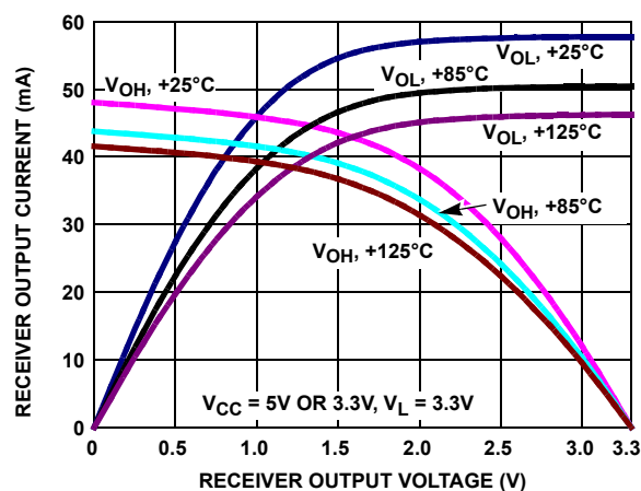
FIGURE 11. ISL3217xE RECEIVER OUTPUT CURRENT vs RECEIVER OUTPUT VOLTAGE
