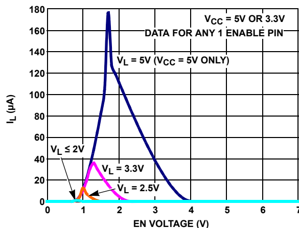
FIGURE 9. V_L SUPPLY CURRENT vs ENABLE PIN VOLTAGE (ISL32x77E ONLY)
