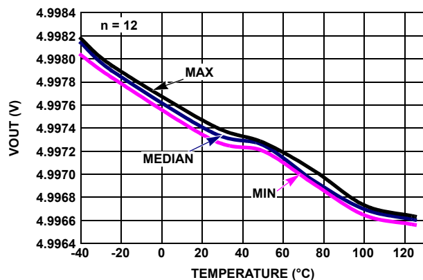
FIGURE 32. V_{OUT} HIGH vs TEMPERATURE, V_+ = 5V , V_- = 0V , V_{CM} = 2.5V , R_L = 100k
