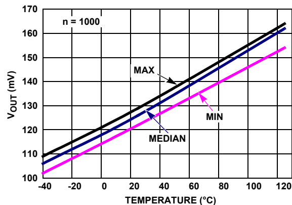
FIGURE 33. V_{OUT} LOW vs TEMPERATURE, V_+ = 5V , V_- = 0V , V_{CM} = 2.5V , R_L = 1k
