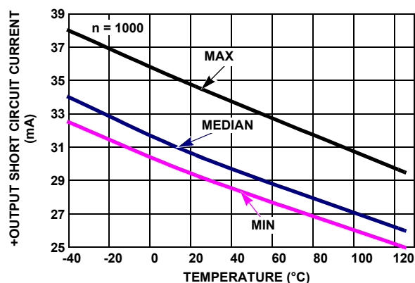
FIGURE 35. +OUTPUT SHORT CIRCUIT CURRENT vs TEMPERATURE V_{IN} = +2.5V , R_L = 10 , V_+ = 5V , V_- = 0V , V_{CM} = 2.5V
