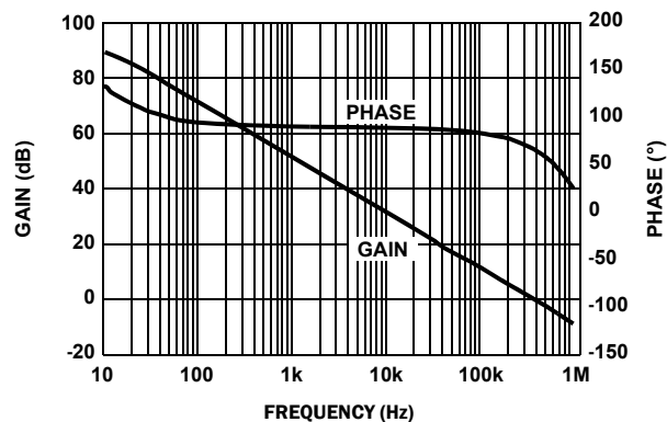
FIGURE 5. A_{VOL} vs FREQUENCY @ 1k \Omega LOAD
