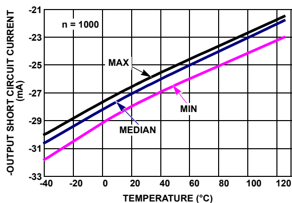
FIGURE 36. -OUTPUT SHORT CIRCUIT CURRENT vs TEMPERATURE V_{IN} = -2.5V , R_L = 10 , V_+ = 5V , V_- = 0V , V_{CM} = 2.5V
