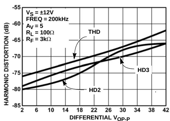
FIGURE 32. HARMONIC DISTORTION vs DIFFERENTIAL OUTPUT VOLTAGE ( 3/4 I_S )
