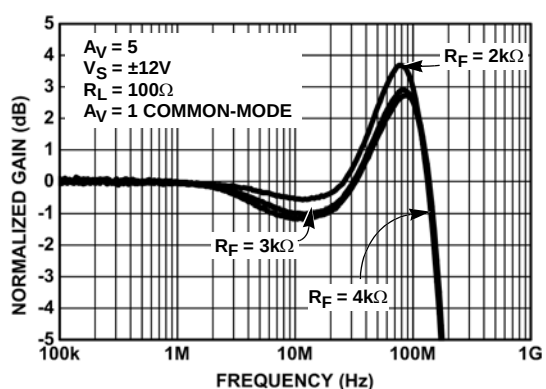
FIGURE 12. COMMON-MODE FREQUENCY RESPONSE vs R_F ( 1/2 I_S )
