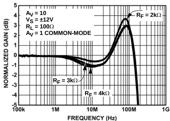
FIGURE 6. COMMON-MODE FREQUENCY RESPONSE vs R_F ( 1/2 I_S )
