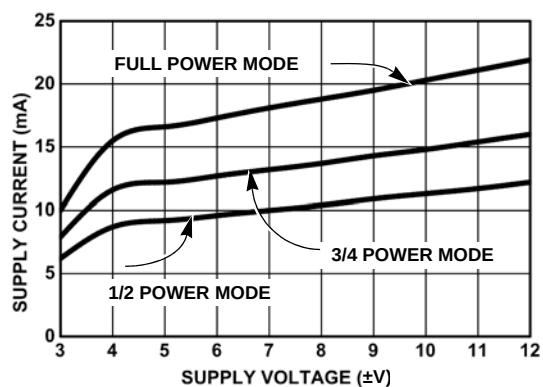
FIGURE 34. SUPPLY CURRENT vs SUPPLY VOLTAGE
