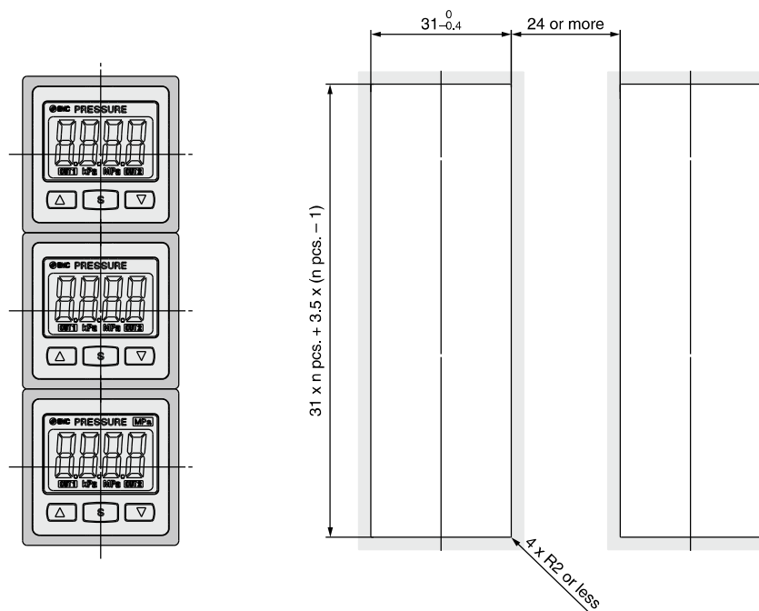
Multiple (2 pcs. or more) vertical mounting
